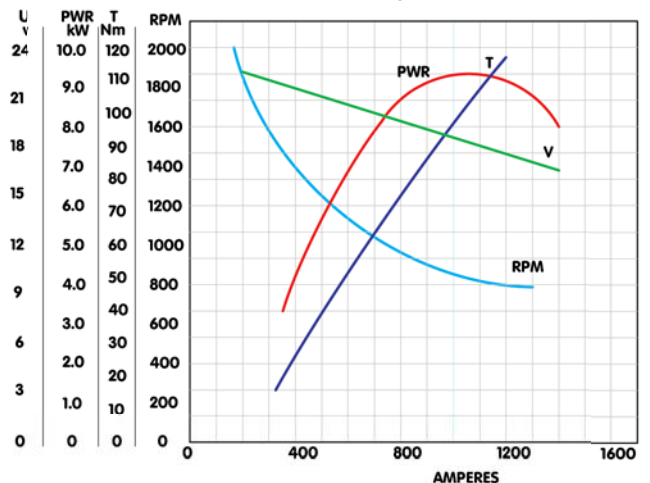
PERFORMANCE CURVES 24V, 9.0 kW
